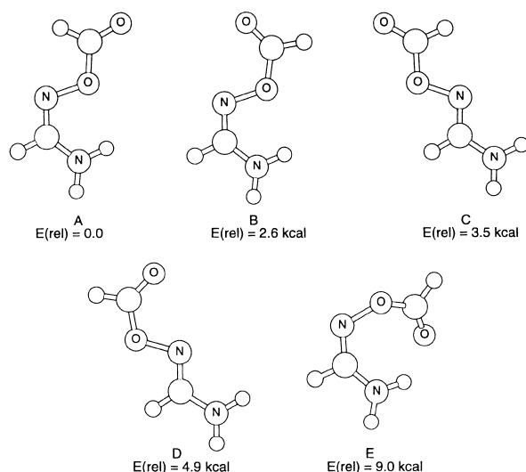
Figure 1. 6-31G*//3-21G conformational energy minima of 2 .
