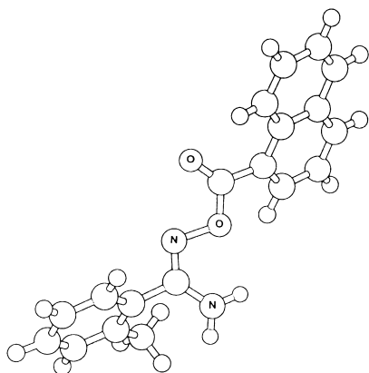
Figure 3. Crystal structure of compound 36 .
